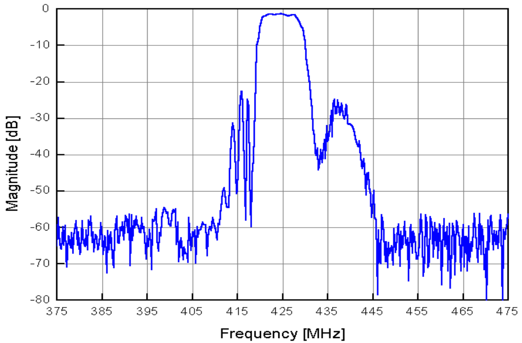
Frequency Response
